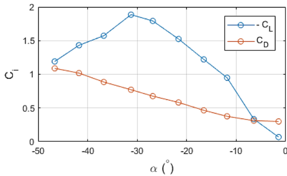
Figure 2. Variation of the negative lift and drag coefficients with the angle of attack obtained with wind tunnel force experiment for U_\infty = 30 \text{ m/s} .
