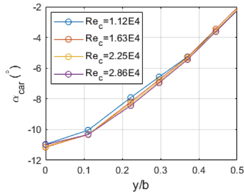
Figure 1. Deflexion of the flow induced by the car along the span for different Reynolds numbers.
