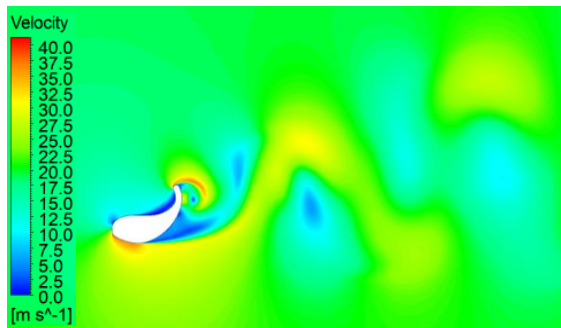
Figure 4. Velocity field in a particular time instance obtained with the numerical model SST k - \omega at \alpha = -30.5^\circ and U_\infty = 20 \text{ m/s} .
