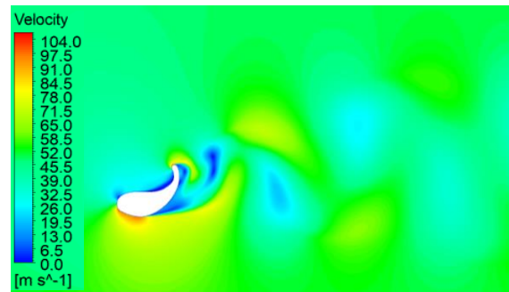
Figure 5. Velocity field in a particular time instance obtained with the numerical model SST k - \omega at \alpha = -30.5^\circ and U_\infty = 50 \text{ m/s} .
