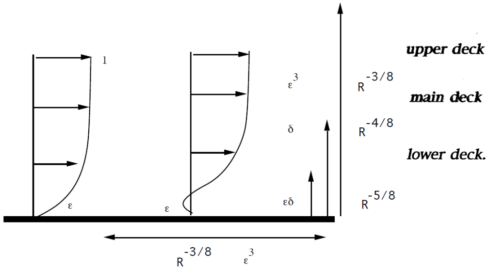
Figure 3.3.2: Illustration of the triple deck theory from Lagr e [50]. The thickness of the lower, main and upper deck are represented.
