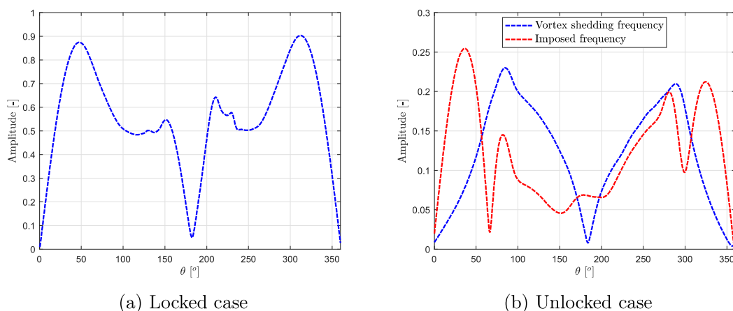
Figure 1: Variations in the amplitude of the main frequency contents in the Fast Fourier Transform of the pressure coefficient around the cylinder's mid-span section at Re = 2.9 \cdot 10^4 : locked (left) and unlocked (right) case
