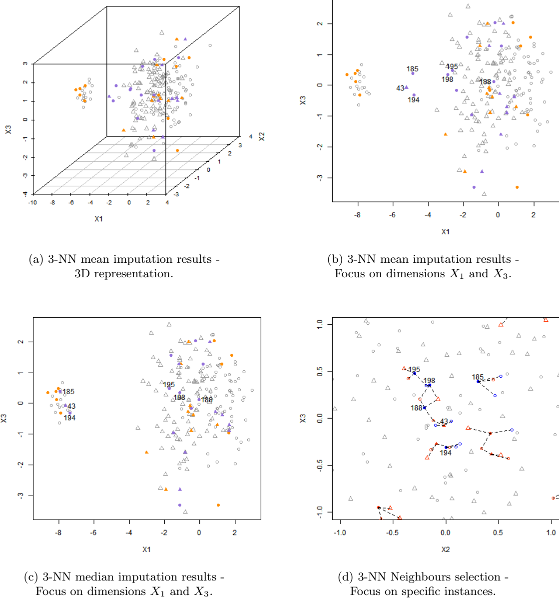
Figure 4.8: Illustration of the 3-NN imputation in configuration n°1 : 10% contamination on X_1 and 10% missingness on X_1 . The red symbols represent the clean missing instances while the blue symbols represent the contaminated missing instances. The red/blue shapes represent the selected neighbours.
