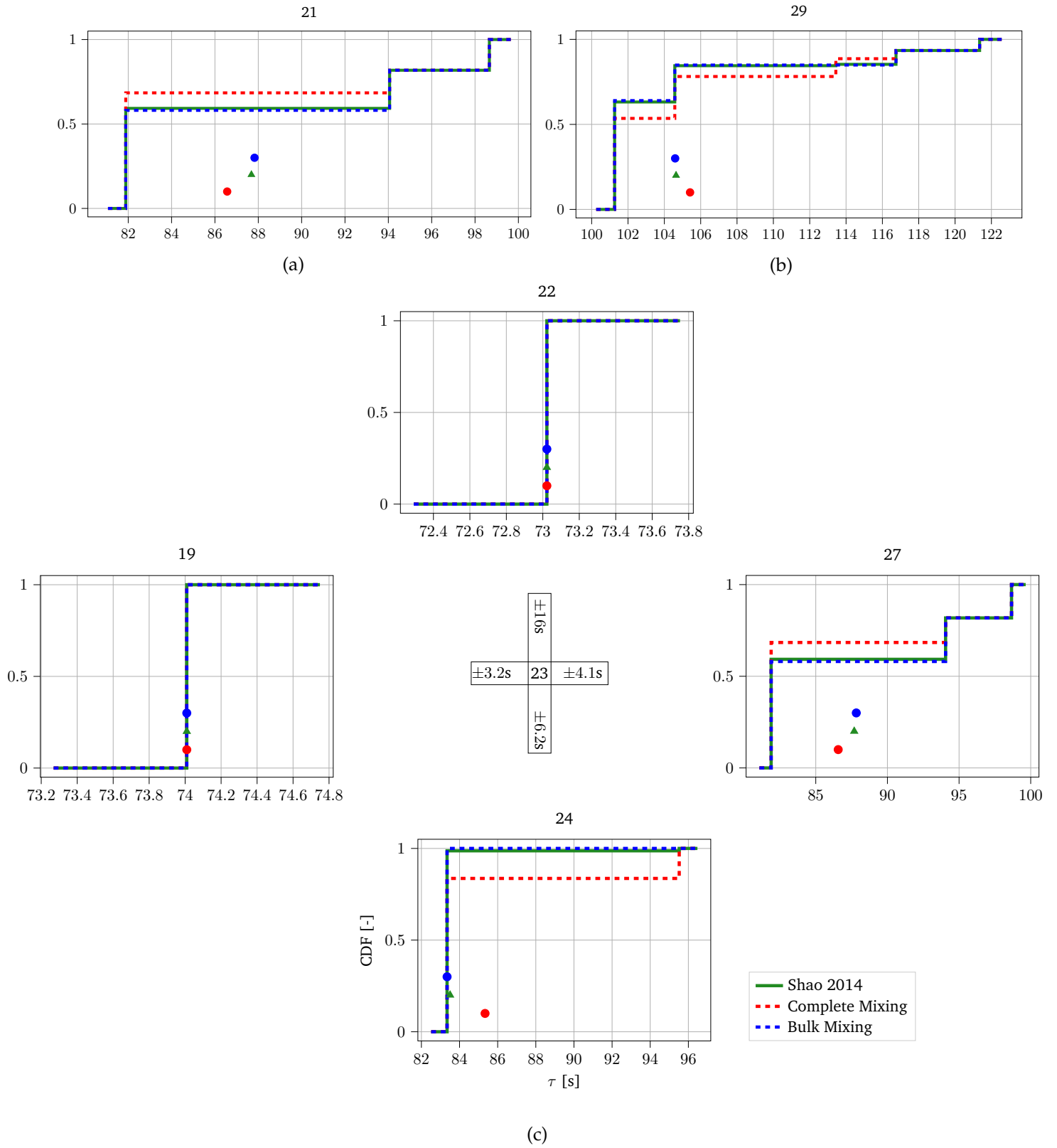
Figure 3.17: Non-homogeneous mixing applied to network Test Rig (Fig. 1.2b). Each figure shows results obtained with complete mixing, bulk-mixing, and flow distribution factors from Shao et al.([29]). Symbols indicates mean ages (at an arbitrary y -coordinate). Figs. 3.17a and 3.17b show the cumulative distribution for junction 21 and 29 respectively. Fig. 3.17c shows a detailed answer for junction 23 and its neighbours.
