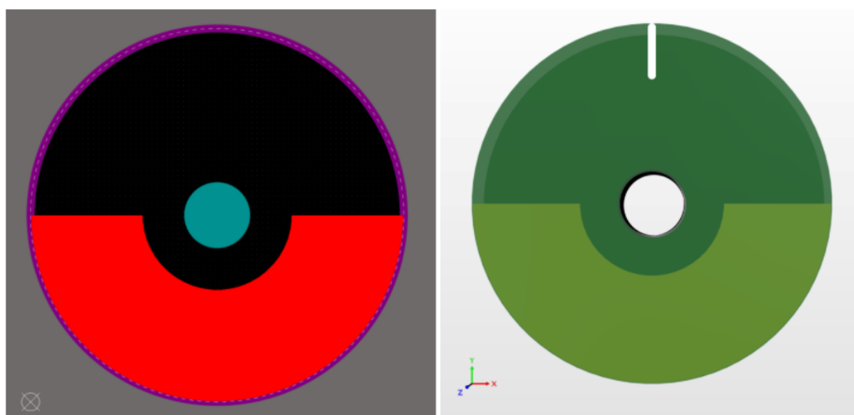
Figure 4.27 – Target design. Left : Top layer of the PCB, right : 3D view
