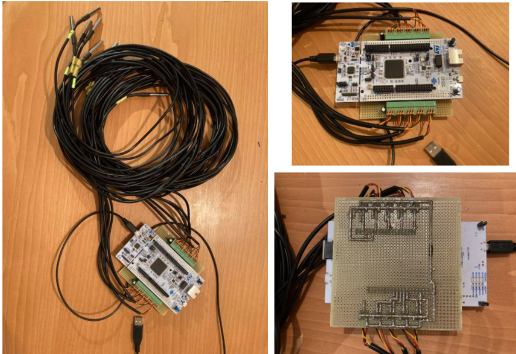
Figure 5.9 – Final design digital thermometer
