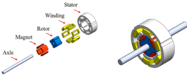
Figure 2.3 – PMSM assembly [4]
