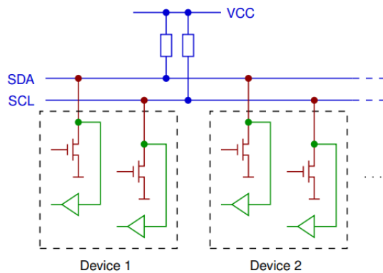
Figure 5.1 – I^2C bus[3]
