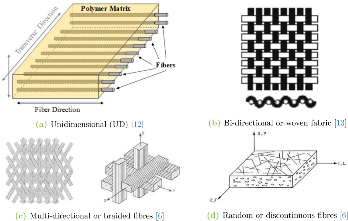
Figure 2.1: fibres arrangement.
