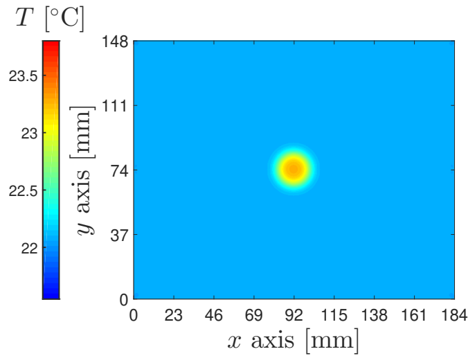
Figure 4.32: Temperature of the upper surface at three seconds with the FBH model.
