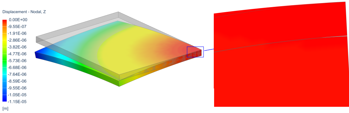
Figure 4.12: Displacements according to z ( w ) of the quarter plate. The image corresponds to deformation at 6 seconds with the conductance set to k'_3 .
