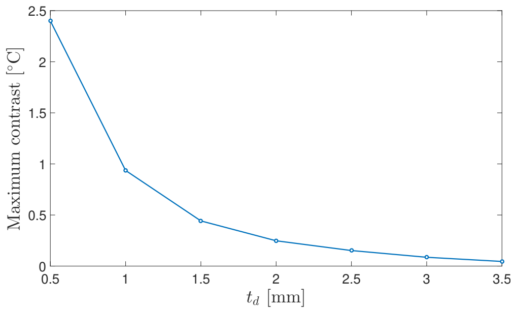
Figure 4.39: Maximum contrast evolution with defect depth.
