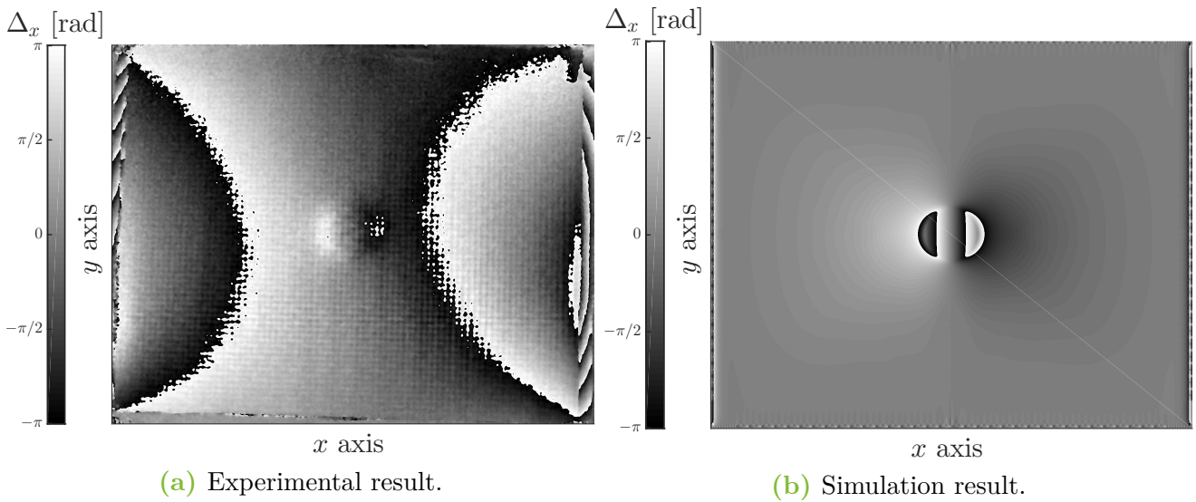
Figure 6.17: Comparison of experimental and numerical simulation phase diagram at 6 seconds with sample \text{FBH}_{\text{free}} ( \delta x = 0.005 m).
