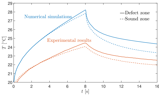
Figure 6.11: Comparison of temperature time evolution in the defect and a sound zone between experimental and simulation results on sample \text{FBH}_{\text{free}} .
