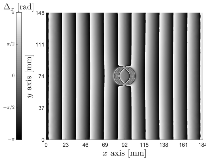
Figure 4.29: Phase diagram, \Delta_x , at 3 seconds. Shear: \delta x = 0.005 m.
