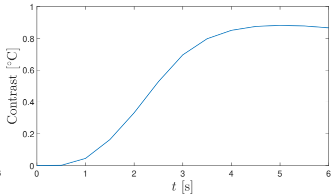
Figure 4.34: Thermal contrast evolution with the FBH.
