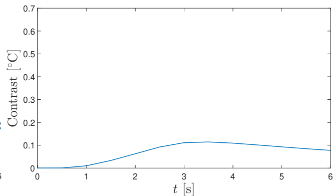
Figure 4.26: Thermal contrast evolution with the Teflon ® layer.
