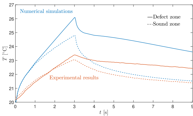
Figure 6.15: Comparison of temperature time evolution in the defect and a sound zone between experimental and simulation results on sample FBH_{clamped} .
