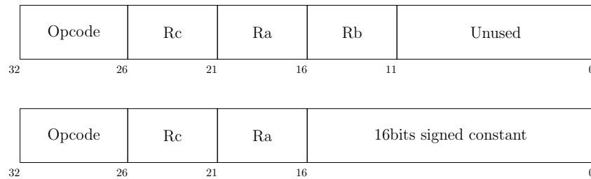
Figure 3.27: Instructions format.
