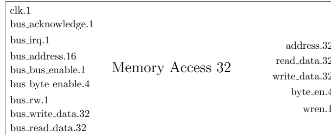
Figure 5.7: Memory Access 32.
