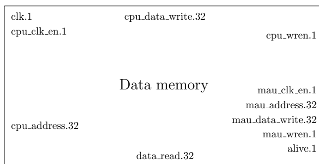
Figure 3.20: Data memory.
