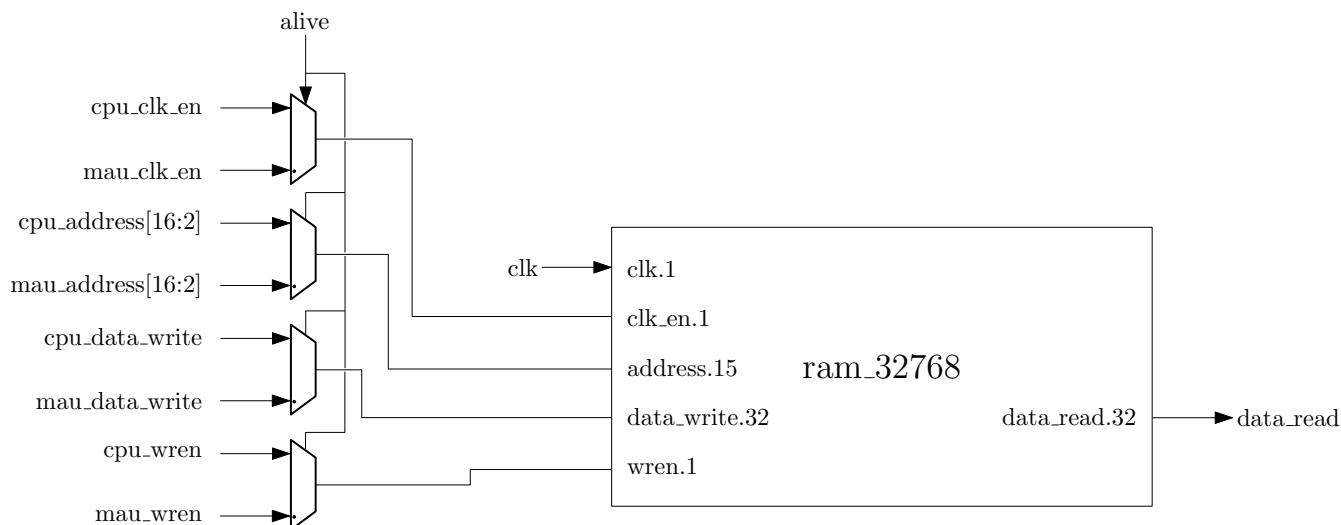
Figure 3.19: Instruction memory internal circuit.
