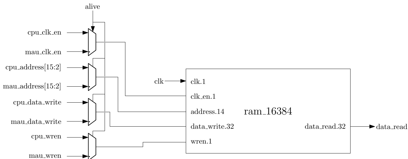
Figure 3.21: Data memory internal circuit.
