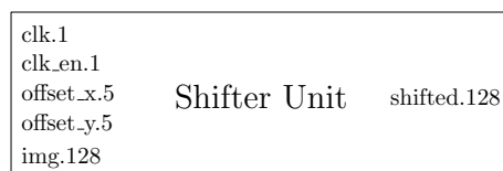
Figure 4.18: Shifter unit.
