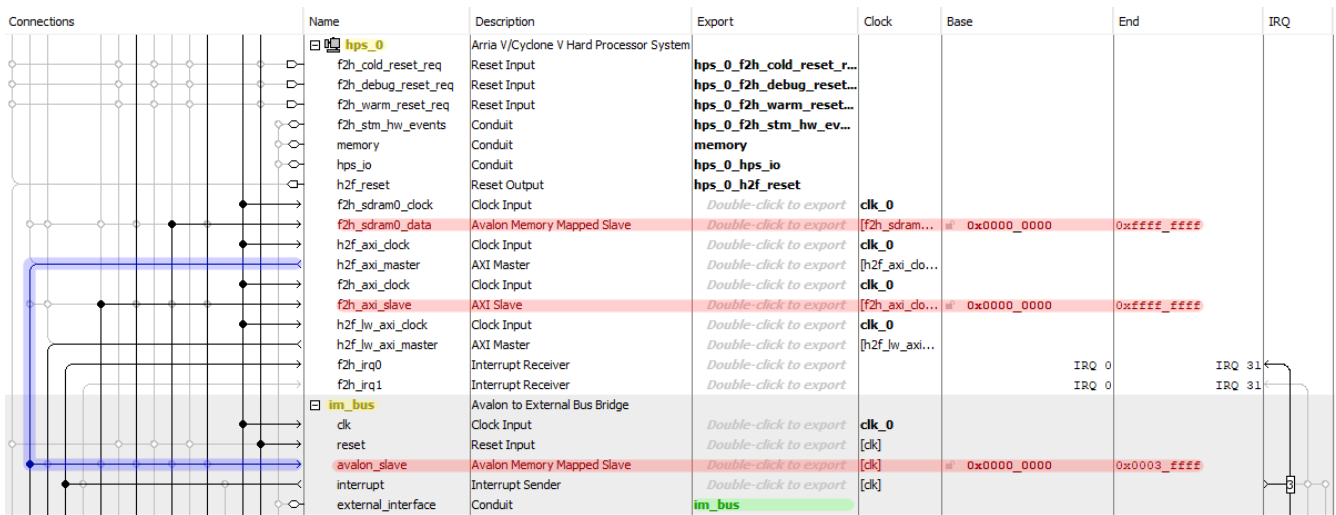
Figure 2.4: QSys window with an HPS named hps_0 and a slave module named mm_bus.
