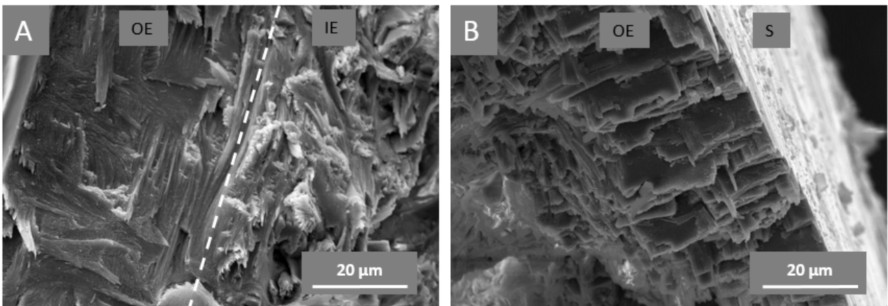
Figure 2: SEM–SE images of frontal section fractures of an oral tooth of the carnivorous P. nattereri . (A) shows the inner and the outer enameloid; (B) shows the outer enameloid. Abbreviations: S , surface; OE , outer enameloid; IE , inner enameloid.
