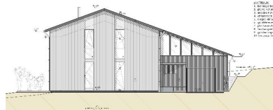
Figure 32 – Façade Est 2
