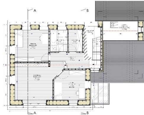
Figure 39 – Plan du +1 3
