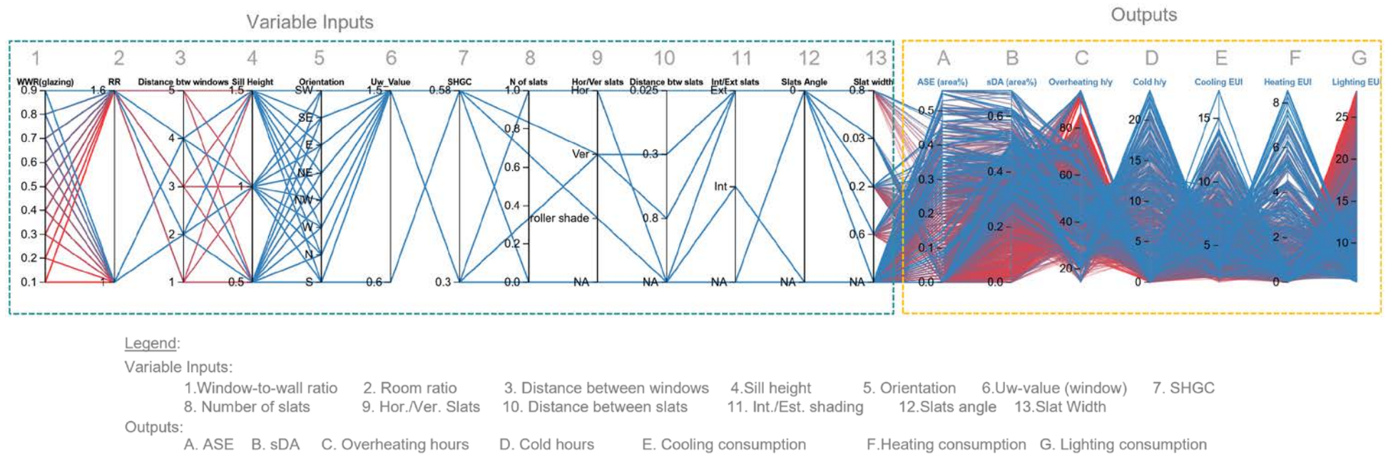
Figure 4-1 Diagram for the different implemented design options
