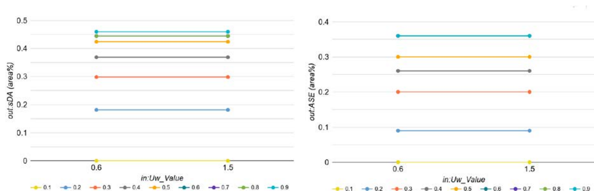
Figure 4-21 The sensitivity analysis results of Uw-value on sDA and ASE regarding the window-to-wall ratio
