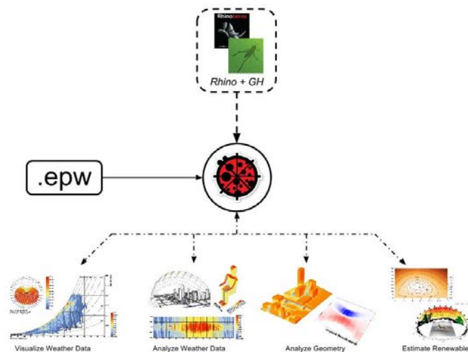
Figure 3-4 Ladybug plugin for Grasshopper- source: ( https://docs.ladybug.tools/honeybee-wiki/ )
