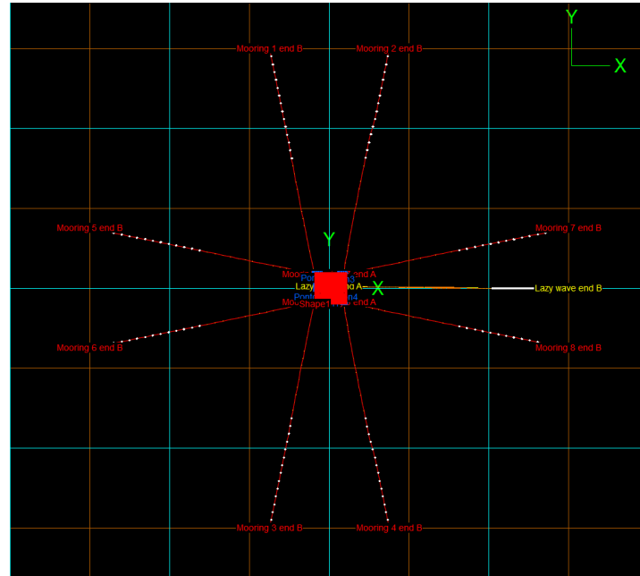
Figure 7.1 Mooring system layout
