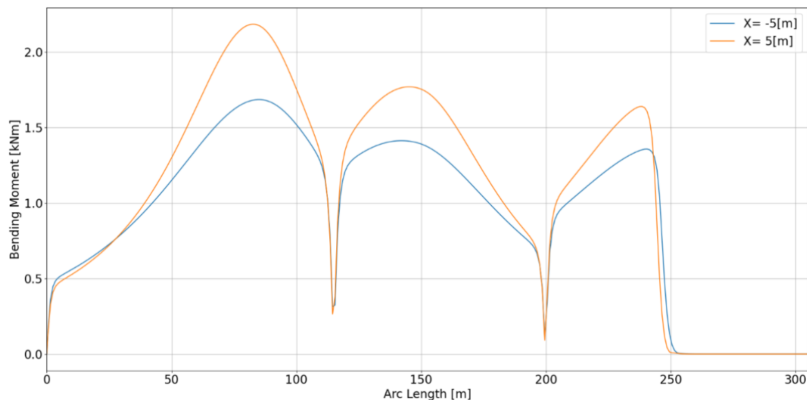
Figure 6.8 Excursion analysis \pm 5 [m]: Bending Moment
