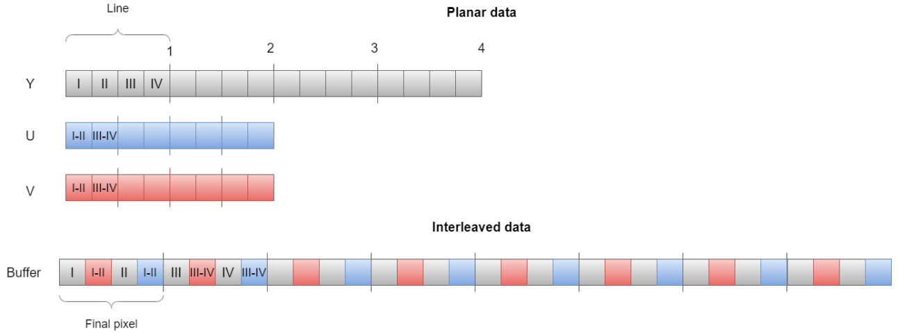
Figure 3.11: Data transformation
