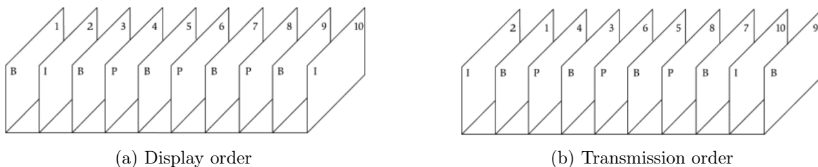
Figure 2.26: GOP structure [2]
