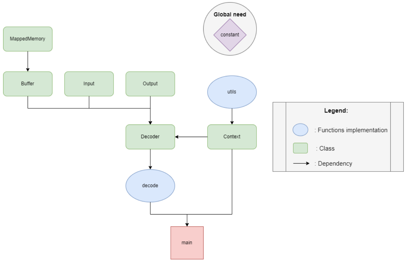
Figure 3.8: Class diagram
