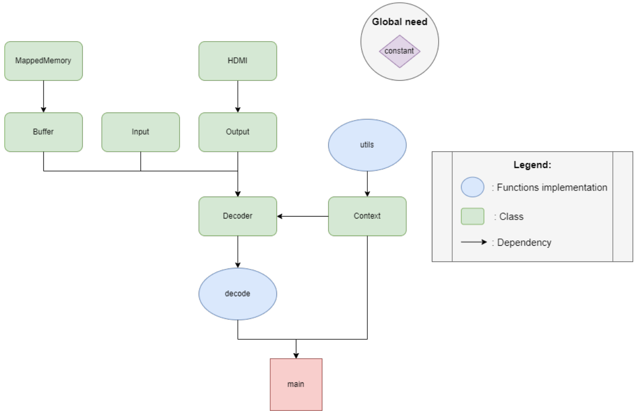
Figure 3.10: Class diagram
