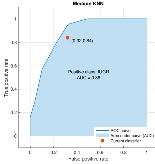
Figure 5.6: ROC curve (blue line) of our Medium K-Nearest Neighbours model. The Area Under the Curve ( AUC = 0.88 ) is the sky blue area and our current classifier performance is the red dot.
