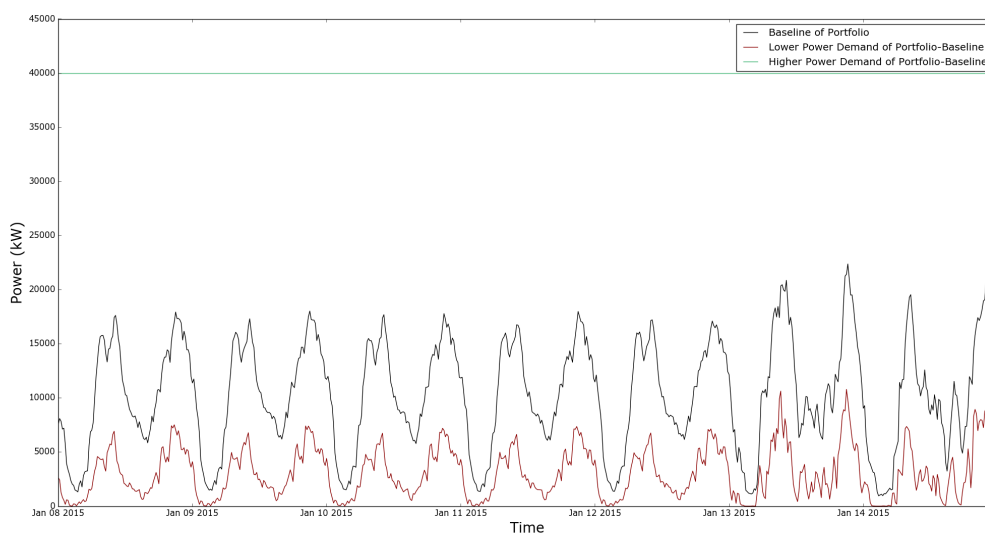
Figure 3.5: Baseline calculated for 10000 tanks and upper/lower power limits.
