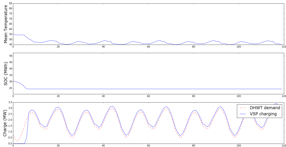
Figure 4.2: VSP state of charge and consumption (2000 tanks).
