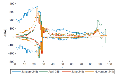
Figure 1.5: Seasonal dependence on activation flexibility [26].
