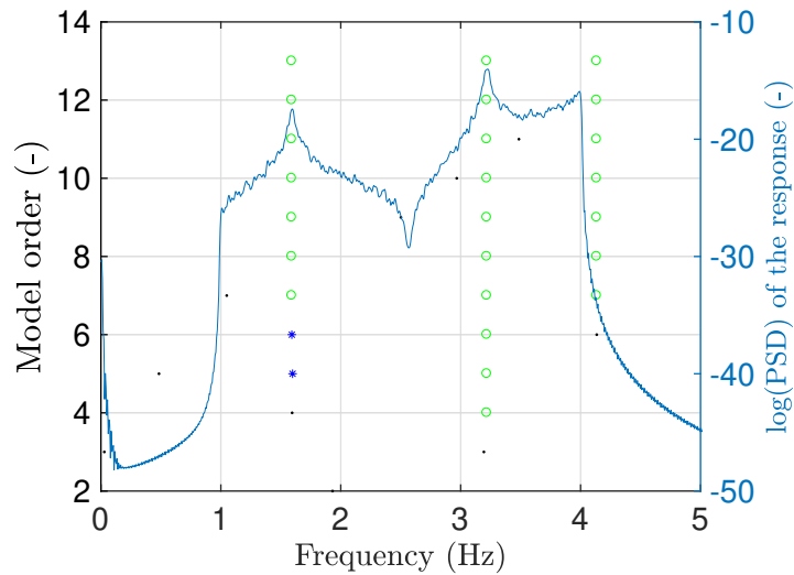
Figure 30: Example of a stabilisation diagram. The green circles represent a pole that stabilised in both frequency and damping ratio while the blue stars mean that the pole only stabilised in frequency. A black dot means that the detected pole neither stabilised in frequency nor in damping ratio.
