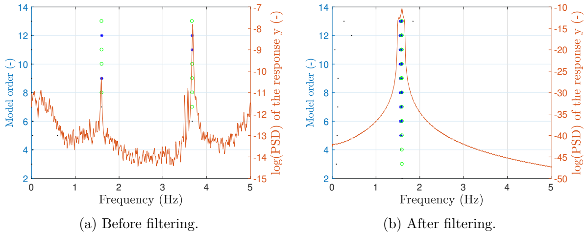
Figure 62: Example of stabilisation diagram for the experimental data, obtained with a random signal from [1 - 7] Hz. In the second figure, the signal is filtered between [1.5 - 1.6] Hz in order to obtain stabilisation at lower orders for mode 1.
