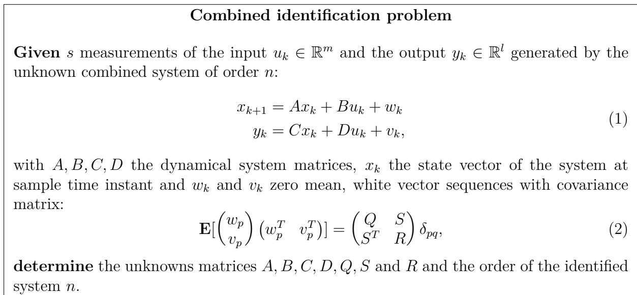
Figure 4: Combined identification problem adapted from [10].
