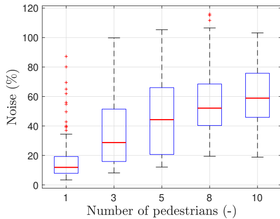
(b) Boxplots.
