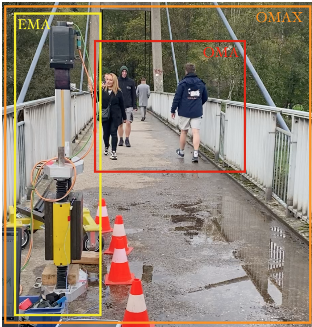
Figure 1: Illustration of the OMAX method being a combination of EMA (uses only artificial forces) and OMA (uses only ambient forces). In this figure, those forces are represented by a shaker and pedestrians respectively.
