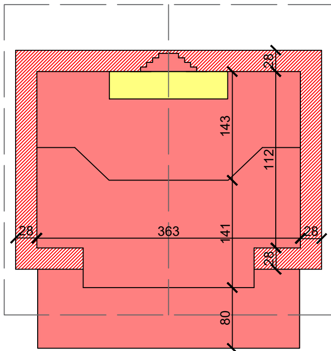
Plan
