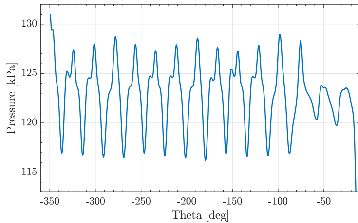
Figure 12: Circumferential profile at rotor exit at 98% of the span height of the pressure only for the nominal blades.
