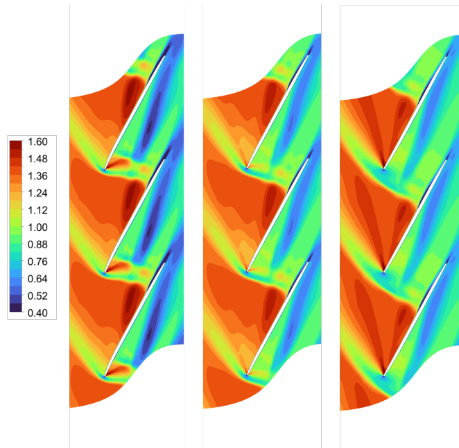
Figure 6: Blade-to-blade plot of the Mach number at 95% of the span of the increased LE curl (left), standard (centre), and decreased LE curl (right) blades.
