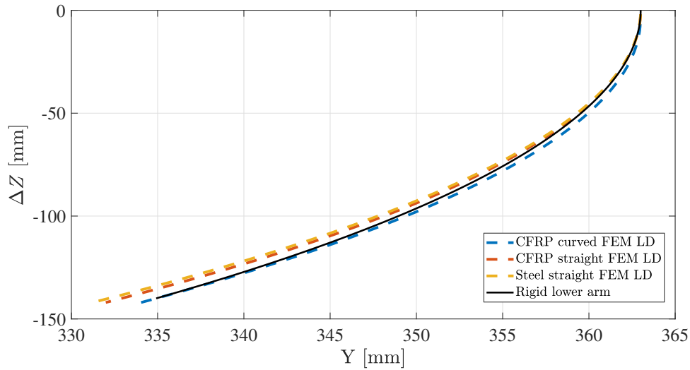
Figure 5.5: Comparison of the lateral deflection Y of the curved leaf spring (integration degree 3) in large deformation (LD) versus lateral deflection of the equivalent straight leaf spring, straight steel leaf of the same length and lateral deflection imposed by a rigid arm..
