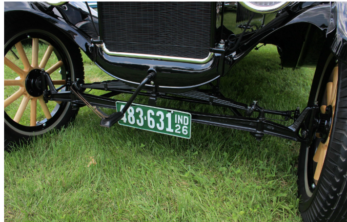
Figure 3: Front suspension of the Ford T[12].
