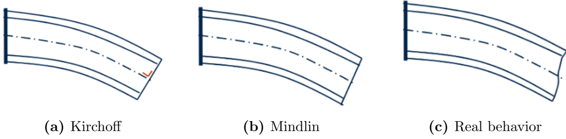
Figure 5.1: Kirchoff assumption (a), Mindlin assumption (b) and real behavior (c) of the section of [36].
