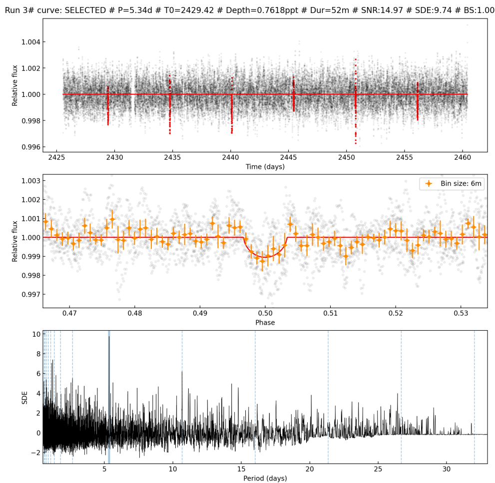
Figure 4.1: EPIC 212465180, SHERLOCK results for the third candidate with a TLS search model. Above: the flux as a function of time and in red lines the suggested transits. Middle: the phase folded curves of the transit. Bottom: the SDE as a function of the Period with the associated harmonics in blue.
