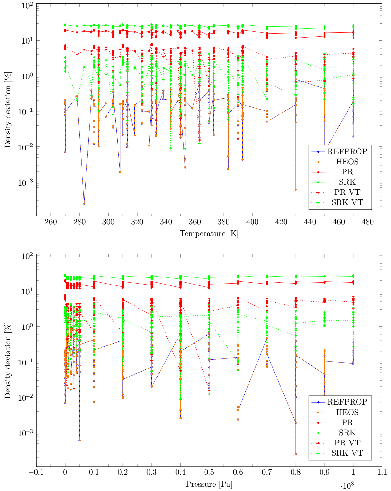
Figure 118: Density dependence on the temperature and pressure for fluid METHYLLINOLEATE
