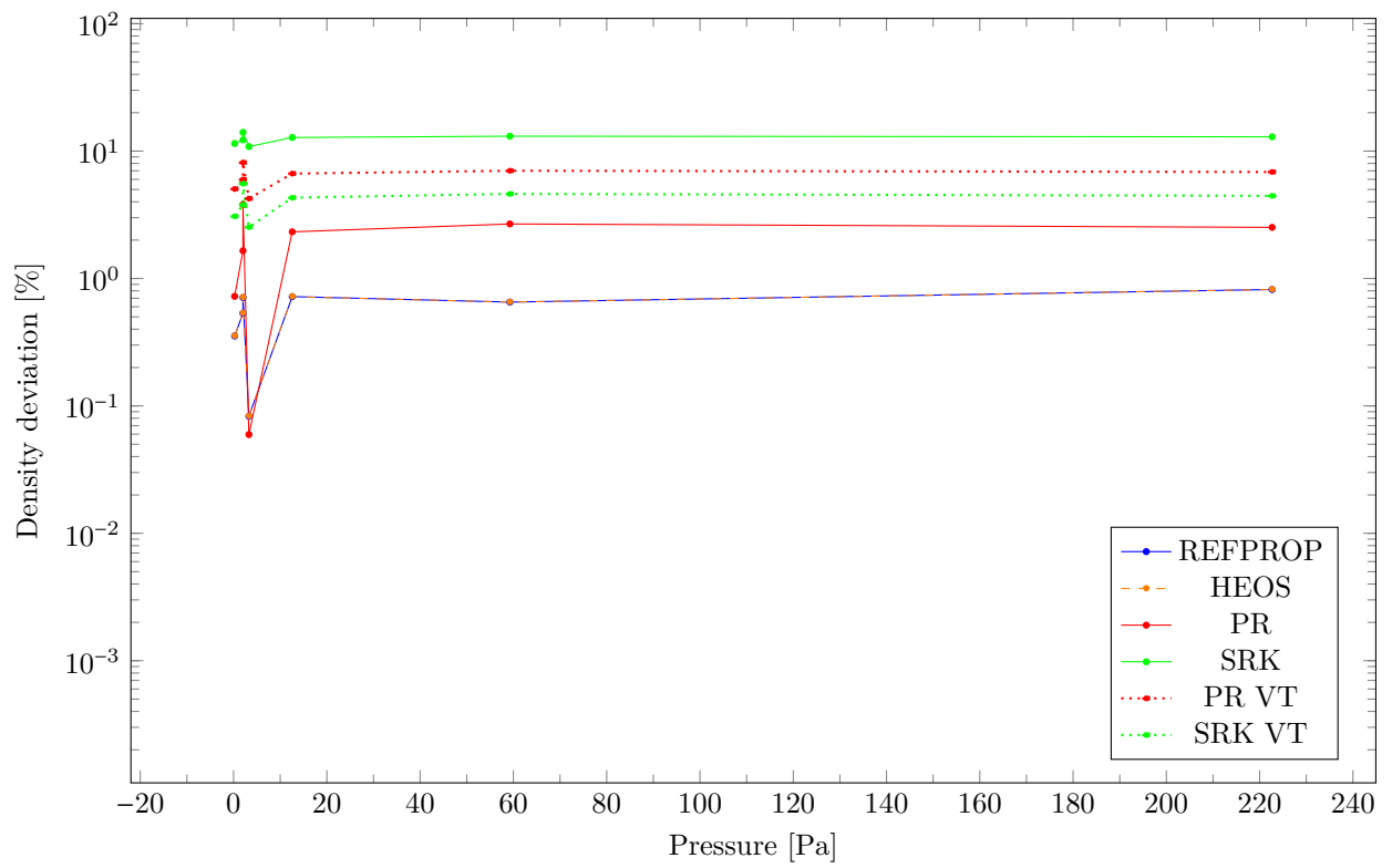
Figure 58: Density dependence on the temperature and pressure for fluid D6
