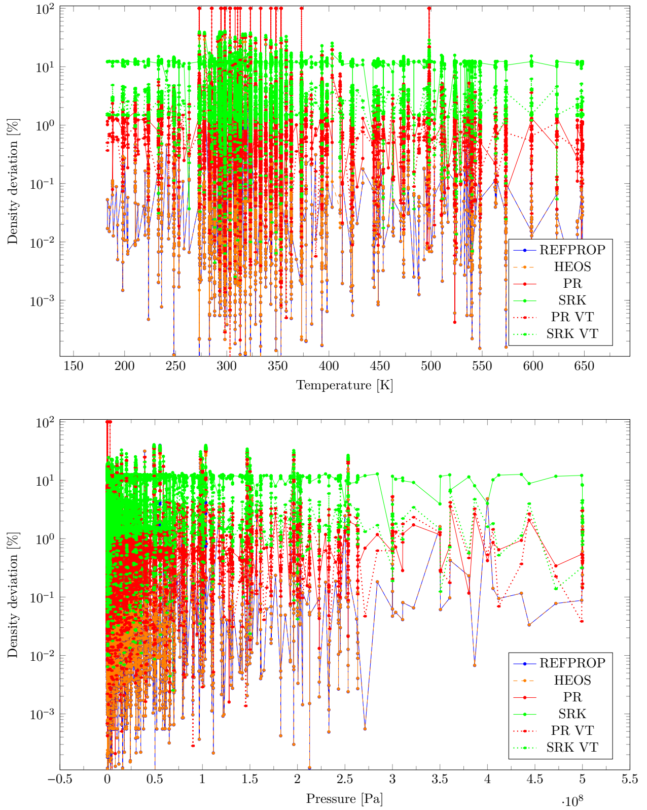
Figure 136: Density dependence on the temperature and pressure for fluid N-HEPTANE
