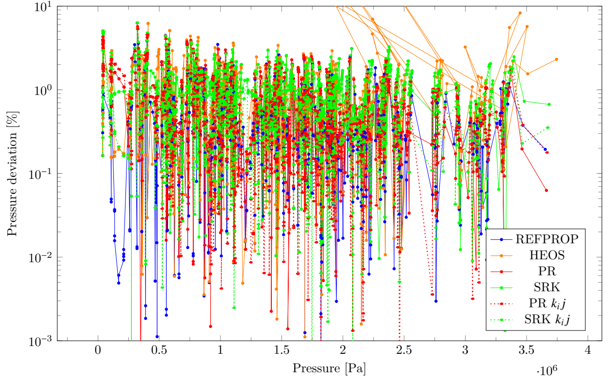
Figure 258: Dependence on the temperature and pressure for the binary mixture R125-R32
