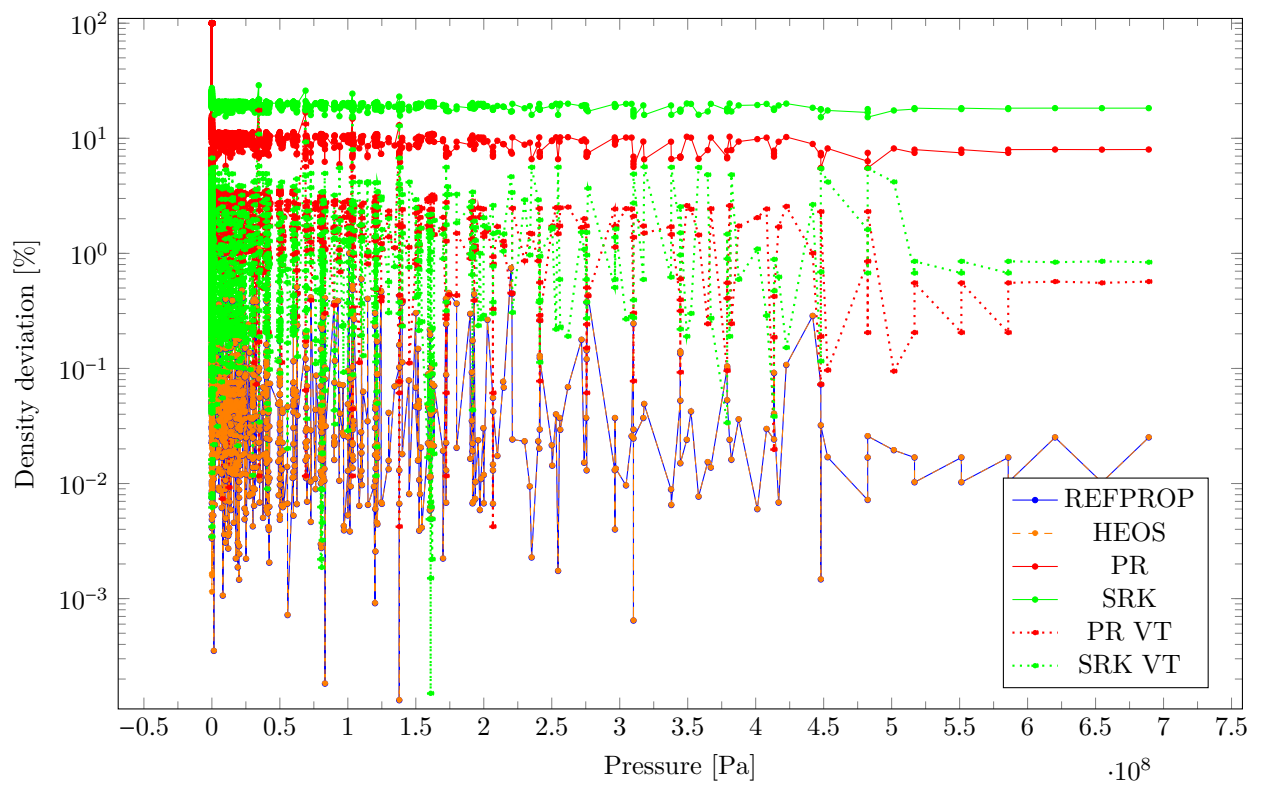
Figure 134: Density dependence on the temperature and pressure for fluid N-DODECANE
