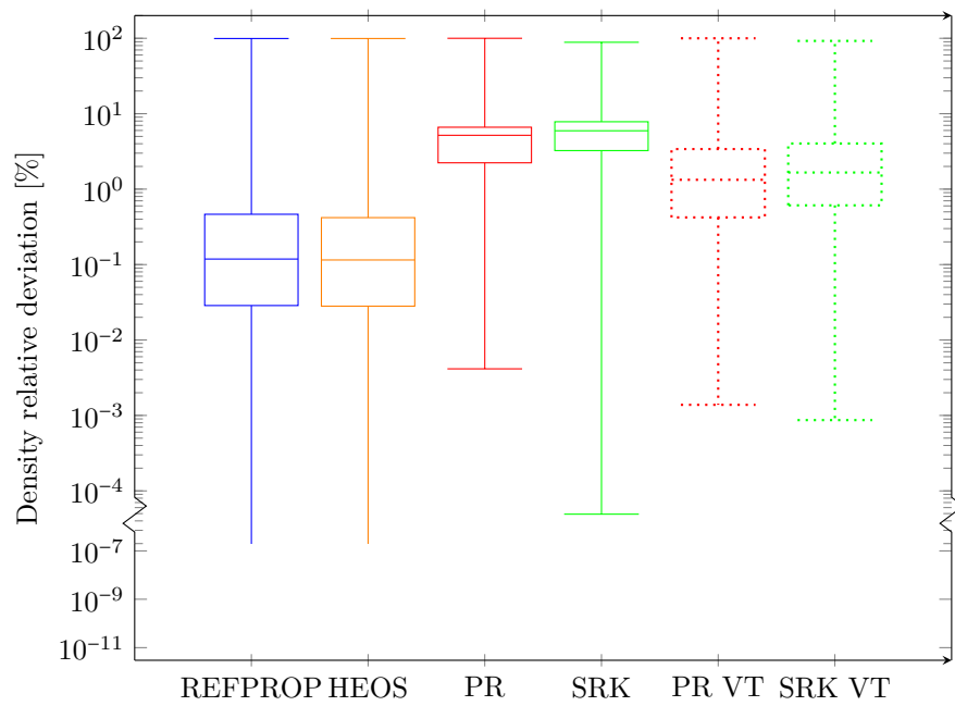
Figure 93: Relative density deviation to experimental data for fluid ISOBUTANE
