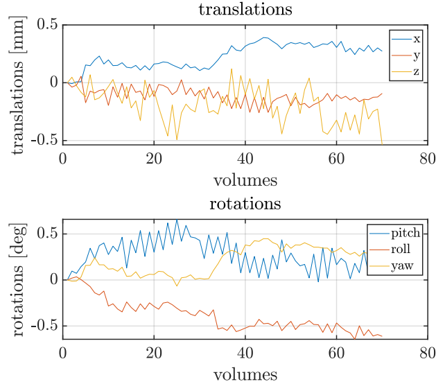
Figure 3.9: Motion parameters of chin task EPI runs of experiment 3.
