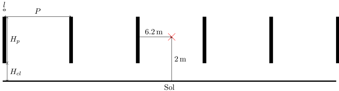
FIGURE 7.6 – Schematic diagram of the Valpuseaux agrivoltaic demonstrator and position of the 3D sonic anemometer within the demonstrator. The red cross indicates the position of the anemometer. P is the pitch distance (10 m). H_p is the panel height (2.087 m). H_{cl} is the clearance height (0.817 m). l is the row width (variable from 3 cm to 10 cm).
