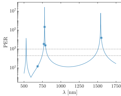
(b) Telecommunication-QKD.
