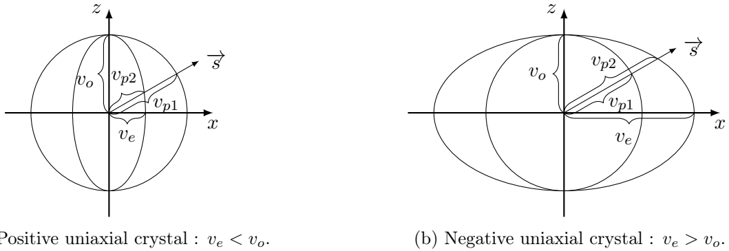
Figure 5.2 – Ellipsoid of wave normals of uniaxial crystals. Adapted from Born and Wolf (1999).
