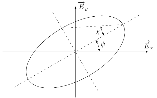
Figure 2.5 – Polarization ellipse. The azimuth angle characterizes the orientation of the principal axis of the ellipse, and the ellipticity angle provides information on the length of the secondary axis, therefore characterizing the phase shift between the components of the electric field.
