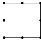
Figure 34: Schematic representation of the element Q8.
