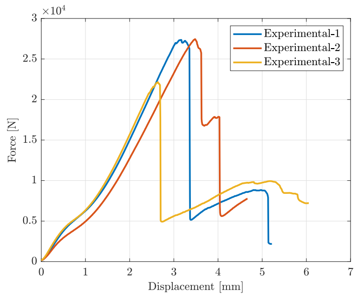
Figure 0.2: Force-displacement curves of experimental data for the hybrid samples 5b. The displacements are normalized.
