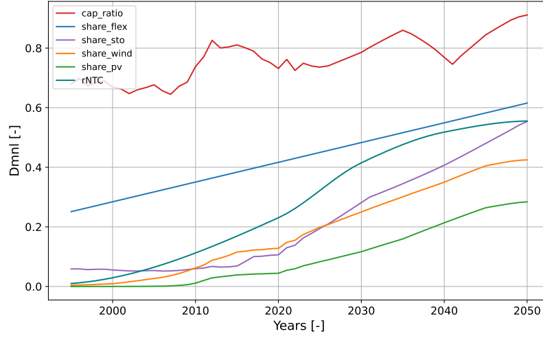
Figure 29: Evolution of the six inputs of the surrogate model in MEDEAS, for the baseline scenario.
