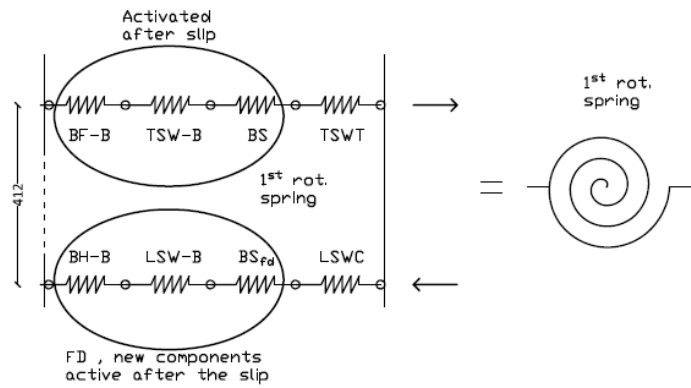
Figure III-8: 1 st rotational spring
