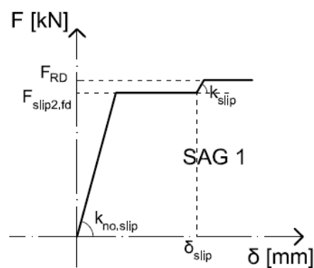
Figure IV-7: F - \delta law of the tensions spring under sagging bending labelled as SAG 1
