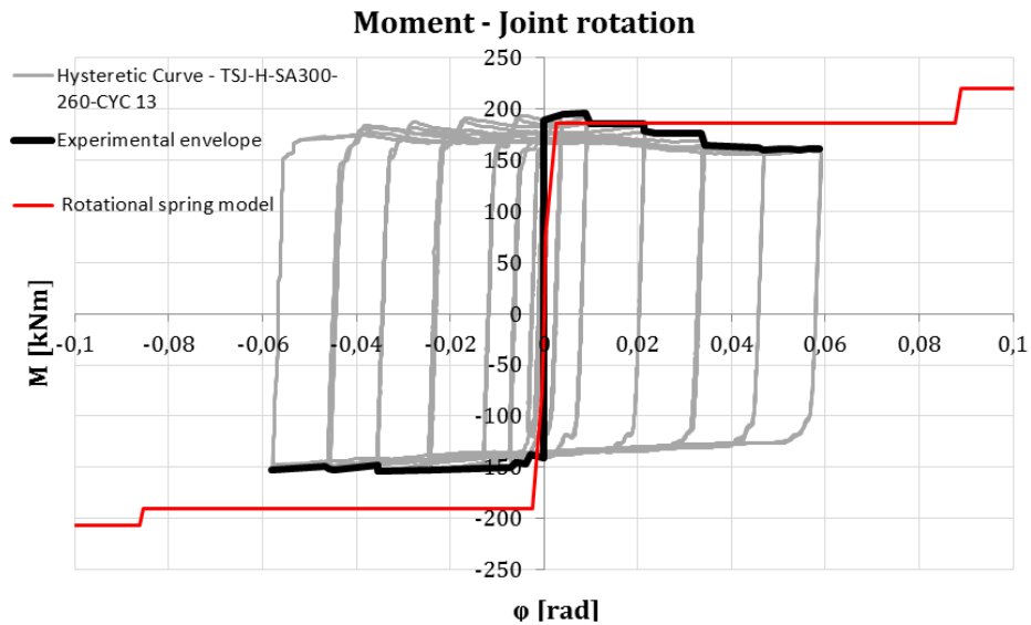
Figure III-14: M-Φ curve of the joint. Rotational spring model. Experimental data.
