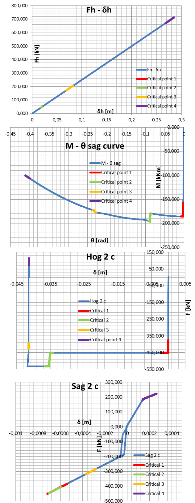
Figure IV-21: Result of the analysis for K_H = 2500
