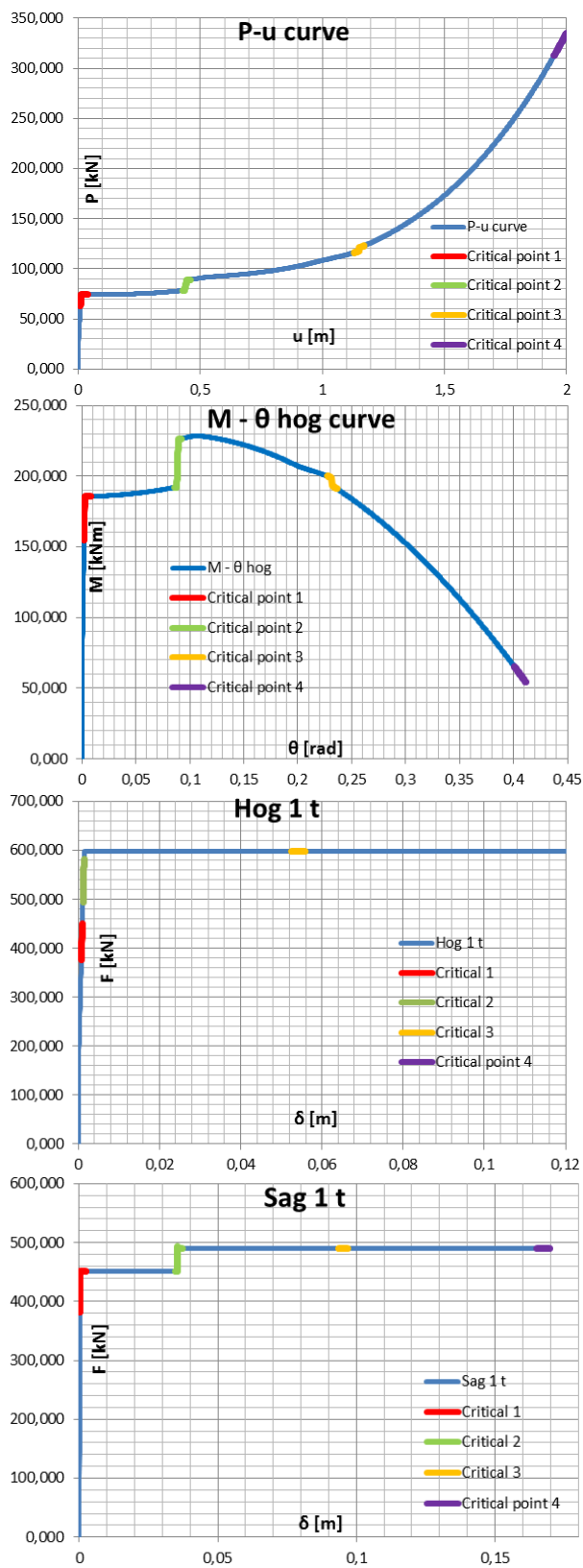
Figure IV-21: Result of the analysis for K_H = 2500
