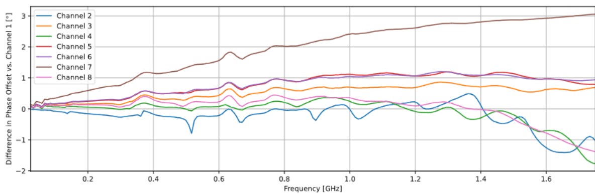
Figure 2: Difference in phase offset between channel 1 and channels 2 through 8 versus frequency.
