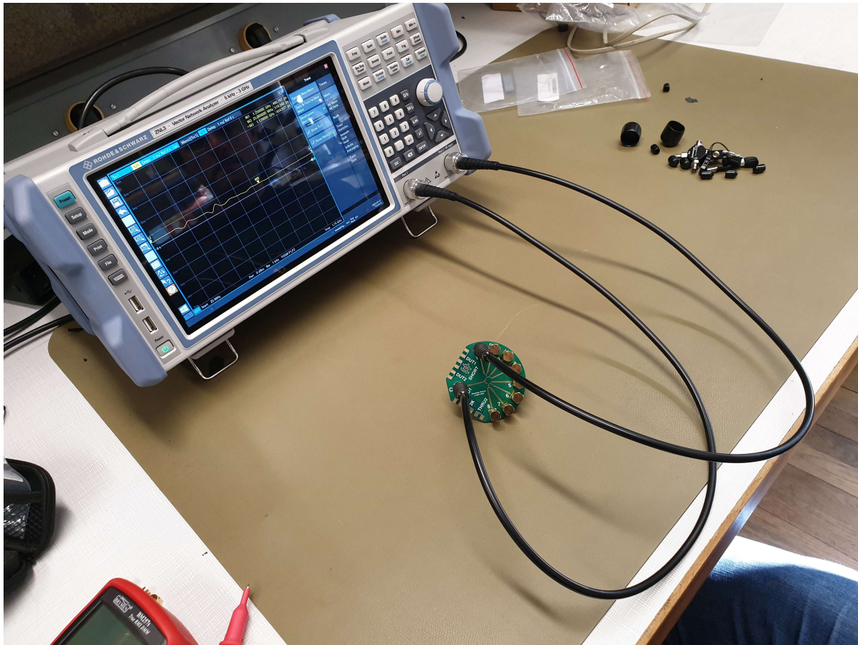
Figure 1: Picture of the test setup used to validate the performance of the phase reference splitter..
