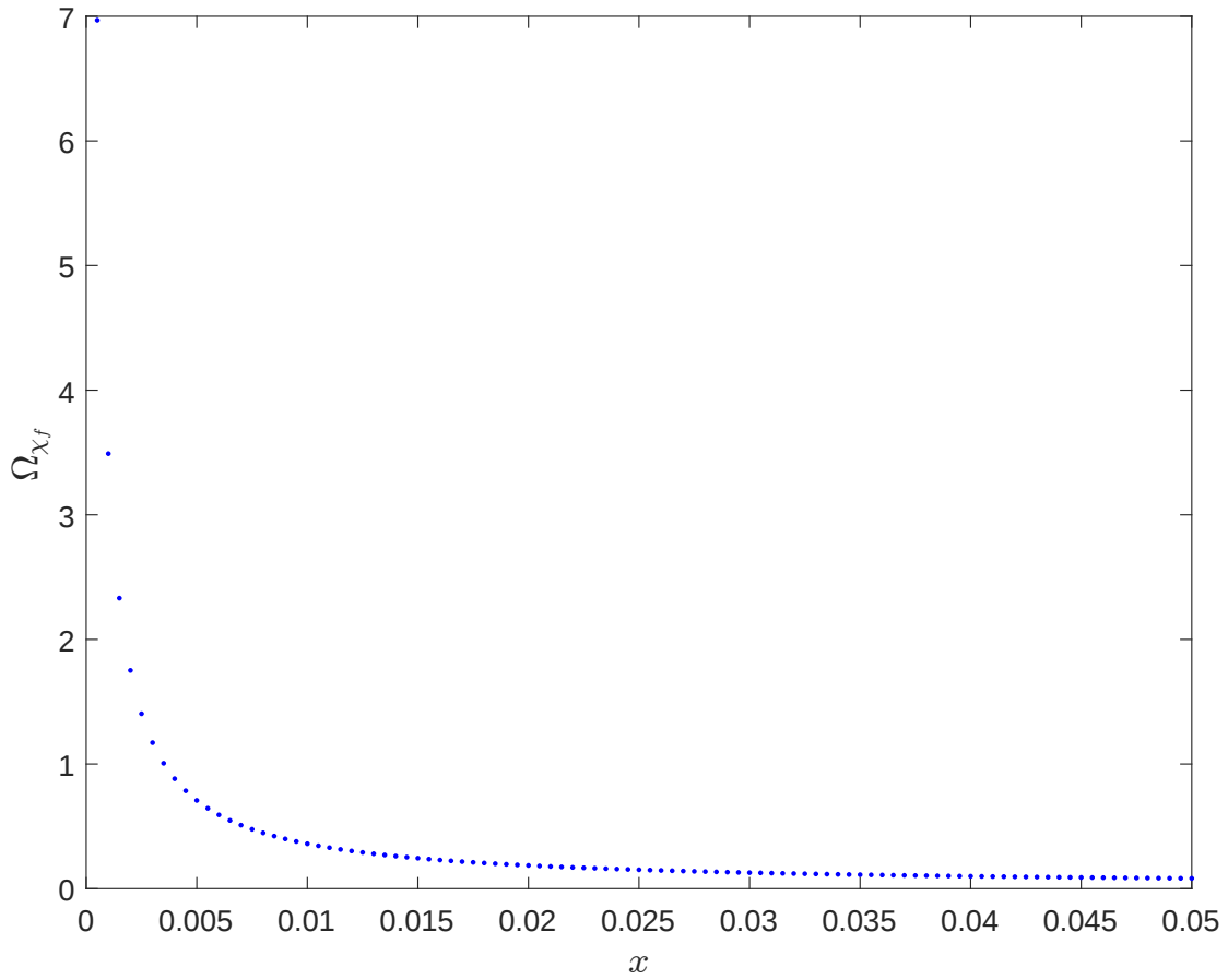
Figure 4.5 – Evolution of \Omega_{\chi_f} as a function of x for M = 500 GeV, m_f = m_e , e = \sqrt{\frac{4\pi}{137}} , g' = 0.9 , n = 0 and 4 g_* = g_{*s} = 86.25 . We see that even if \langle\sigma v_{\text{rel}}\rangle decreases when x increases, it is not automatically the case for \Omega_{\chi_f} which shows a rather fast decrease with x .
