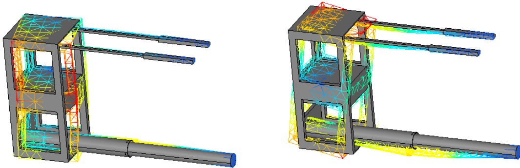
Figure 63: Modes 5 &amp; 6
