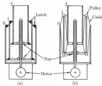
Figure 28: Telescopic motorisation
