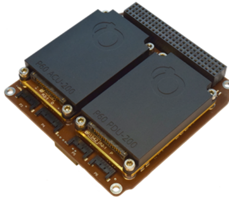
Figure 24: Battery
