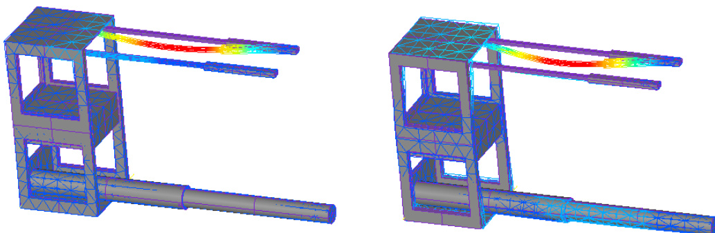
Figure 65: Modes 9 &amp; 10
