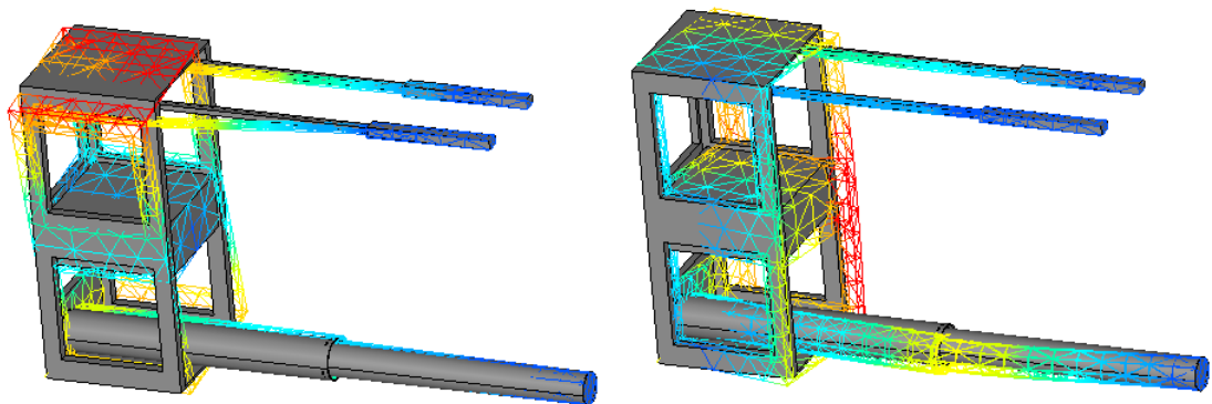
Figure 62: Modes 3 & 4
