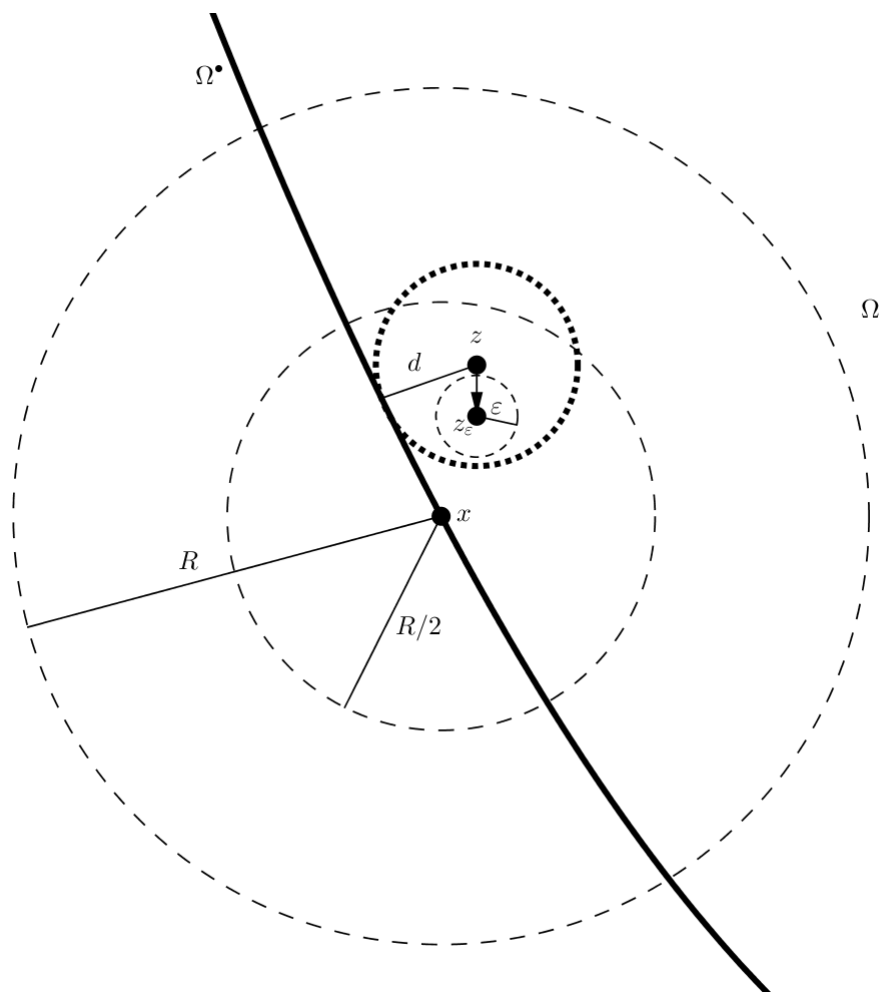
FIGURE A.1 – Construction du point z_\varepsilon .
