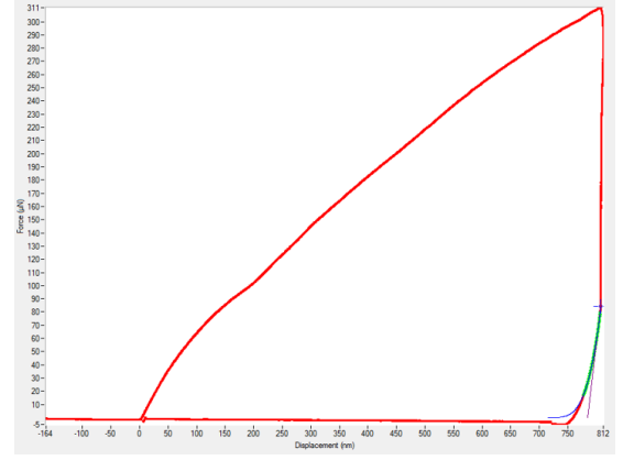
Figure 3.14: Shape of a bad Force-Displacement curve.
