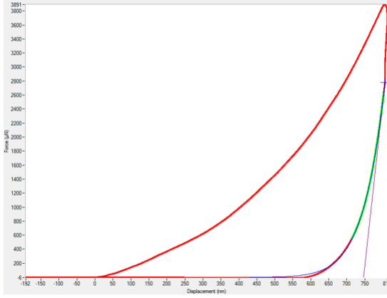
Figure 3.13: Shape of a good Force-Displacement curve.
