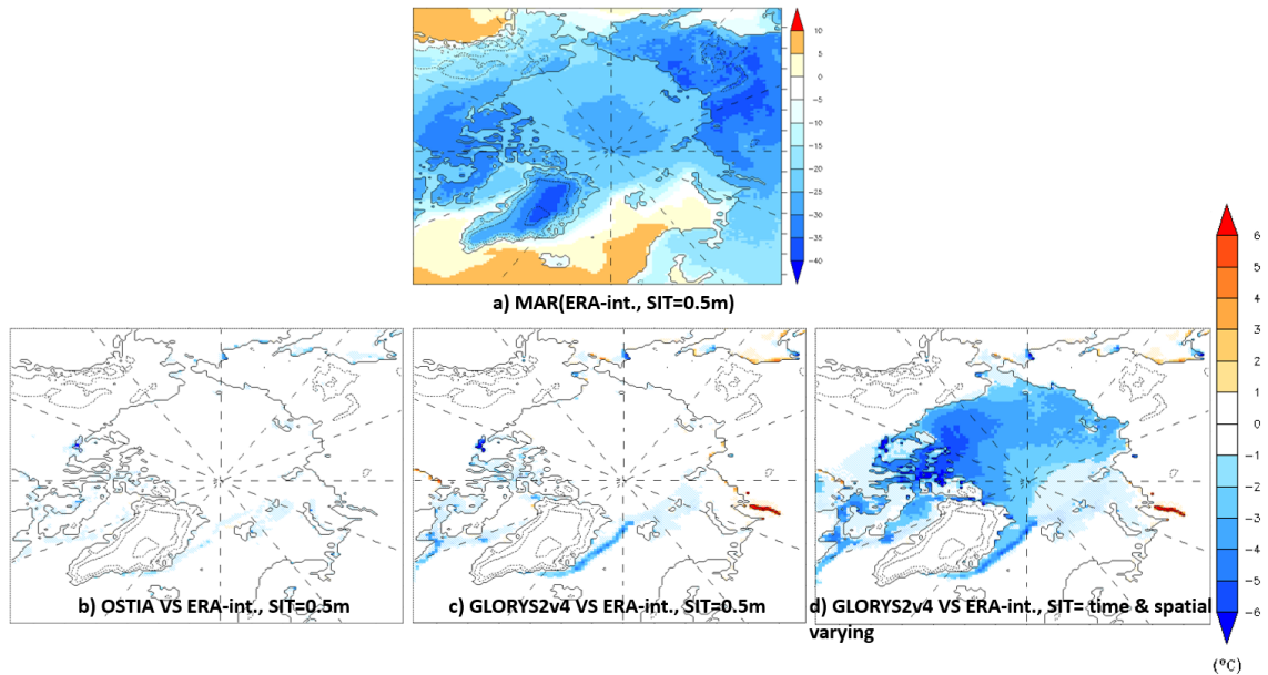
FIGURE 4.2: a) Mean skin temperature for DJF modeled by MAR forced by ERA-interim with 0.5 m SIT over 2000-2015. b to d) Mean skin temperature anomaly for DJF modeled by MAR over 2000-2015. Or MAR(reanalysis=?. SIT=0.5) - MAR(ERA-int., SIT=0.5). (Hatched = insignificant)
