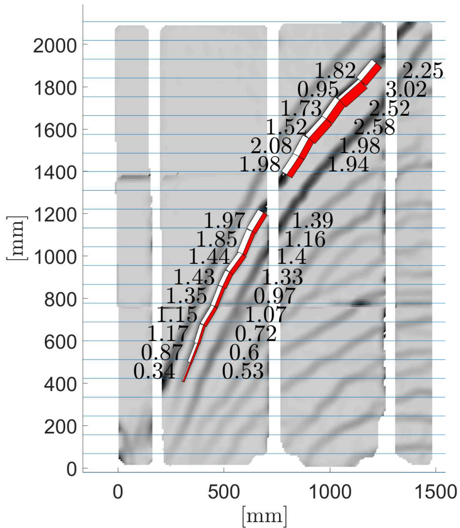
Figure 4.18: Crack width (white) and slip (red) [mm].
