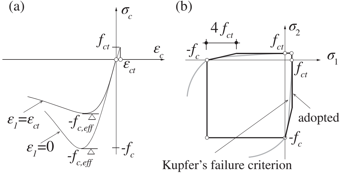
Figure 3.11: (a) Stress-strain diagram for concrete; (b) Kupfer's failure criterion (Kupfer, Hilsdorf, & Rusch, 1969) and adopted one (Cavagnis, Ruiz, & Muttoni, 2018).
