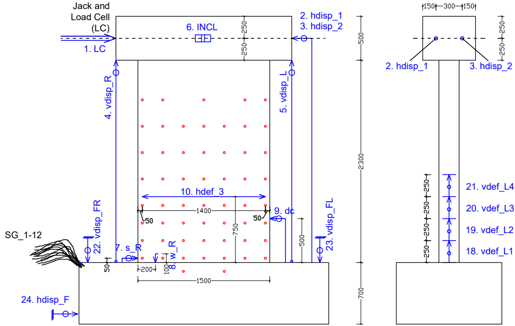
Figure 2.5: Instrumentation (DT sensors, LED targets) of the wall, with compression side view.
