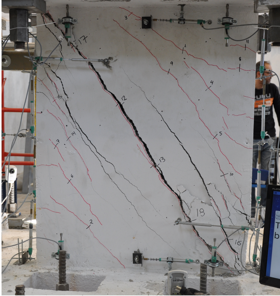
Figure 5.3: Last photograph of the time-lapse (end of test) at a horizontal load of 312 kN and a horizontal displacement of 24.1 mm.
