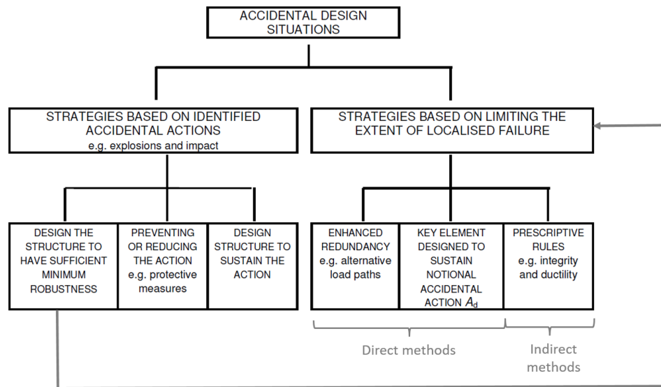
Figure 1.4 – Strategies to reduce the risk of an accidental event with a relatively low probability of appearance [2].
