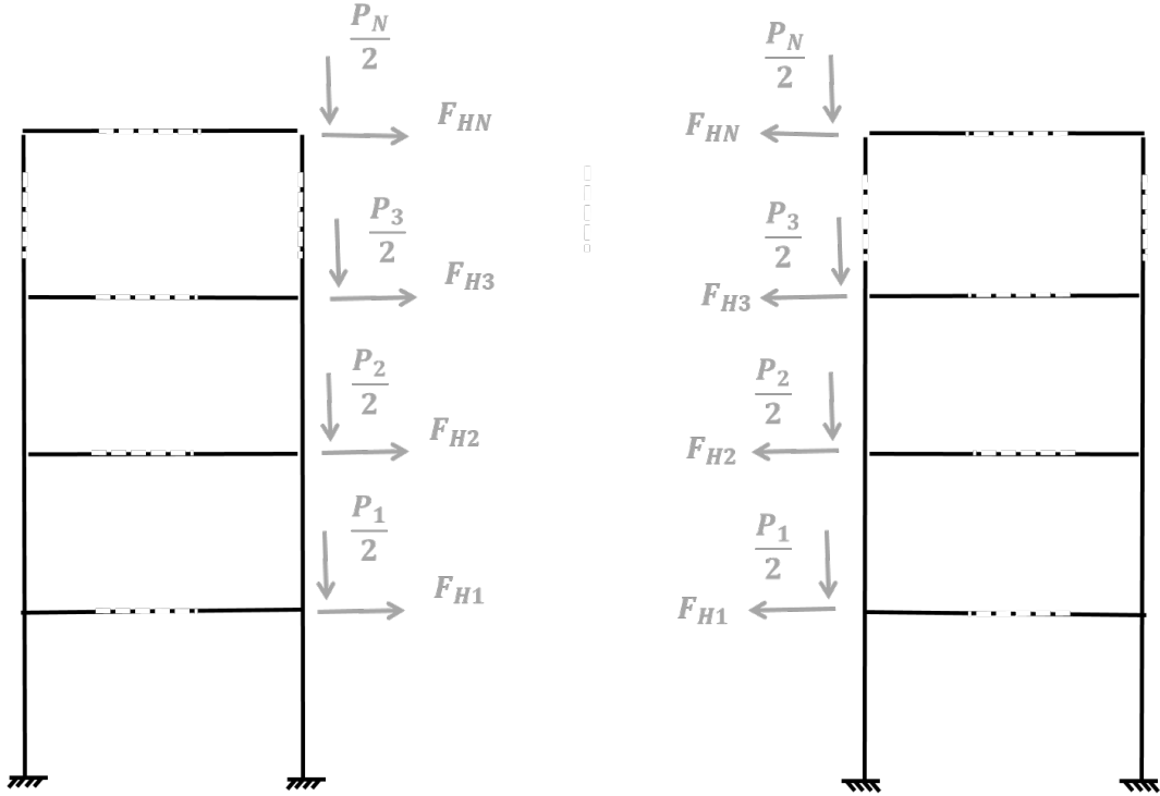
Figure 5.2 – Illustration of the IAP and the DAP reaction forces applied to the IAP during phase 3; where F_{Hi} and \frac{P_i}{2} are respectively the horizontal and vertical reaction forces of the story i of the DAP on the story i of the IAP.
