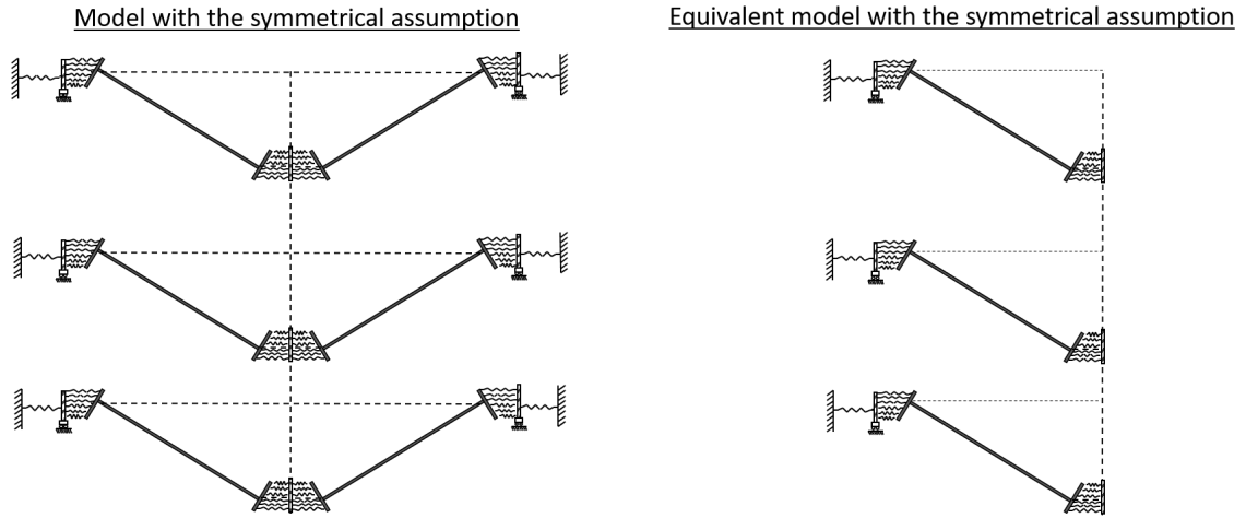
Figure 2.6 – At the left, studied substructure with the symmetrical displacements hypothesis. At the right, studied substructure with the assumptions that the displacements are symmetrical and the beams of each story of the substructure are identical.
