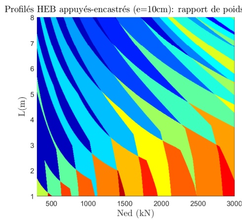
(c) HEB, appuyés-encastres, e=10\text{cm} , S620
