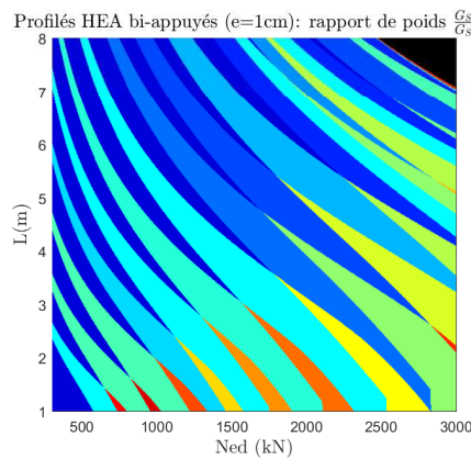
(a) HEA, bi-appuyés, e=1\text{cm} , S500
