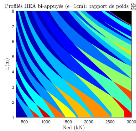
(b) HEA, bi-appuyés, e=1\text{cm} , S550
