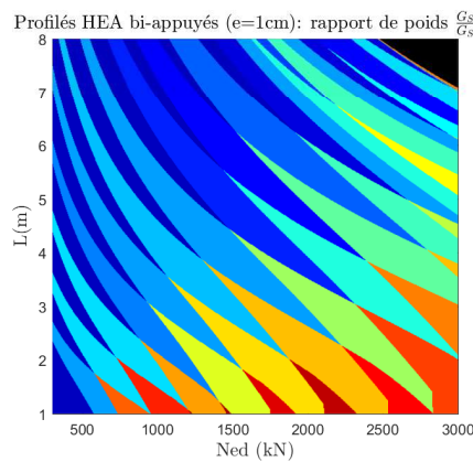
(c) HEA, bi-appuyés, e=1\text{cm} , S620
