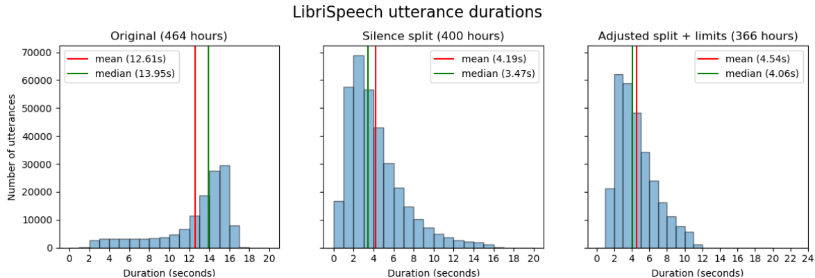
Figure 16: (left) Histogram of the duration of the utterances in LibriSpeech-Clean, (middle) after splitting on silences, (right) after constraining the length and readjusting the splits.
