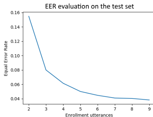
Figure 14: Speaker verification EER on the test set with respect to the number of enrollment utterances. Each speaker is tested against n + 1 utterances used for enrollment.
