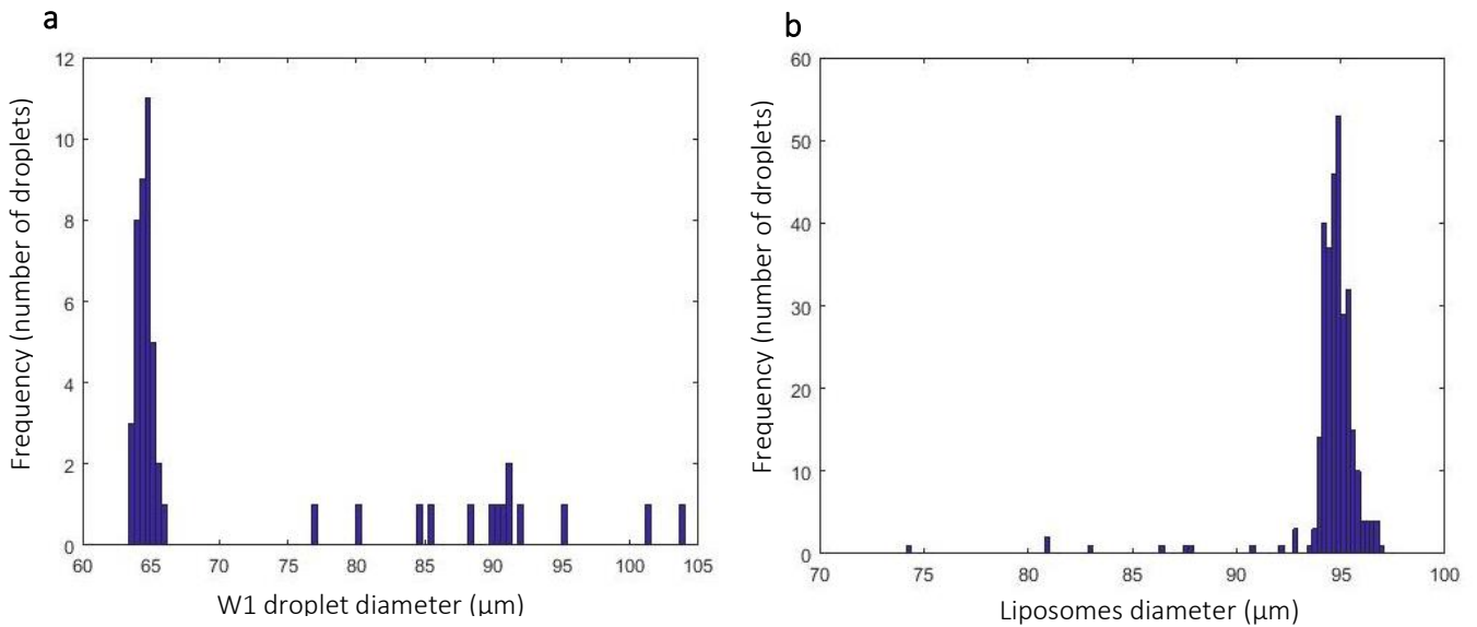
Figure 24 Example of size distribution of (a) W1 droplet ( n=53 ) and (b) liposomes ( n=306 ). The measurement were obtained with Q_{W1}= 0.08 \mu\text{L}\cdot\text{min}^{-1} , Q_0 = 1.02 \mu\text{L}\cdot\text{min}^{-1} and Q_{W2}= 20.45 \mu\text{L}\cdot\text{min}^{-1}
