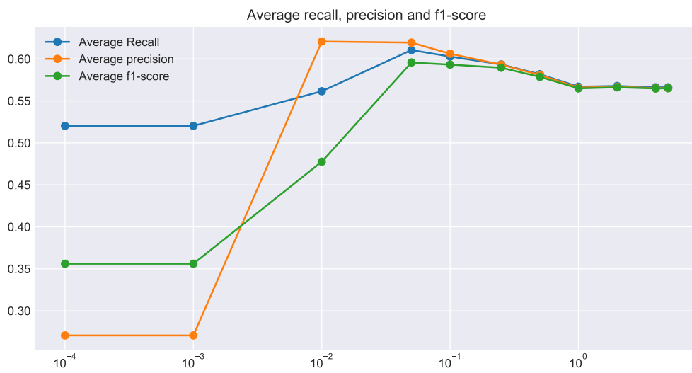
Figure 4.1: Tuning linearSVC parameters
