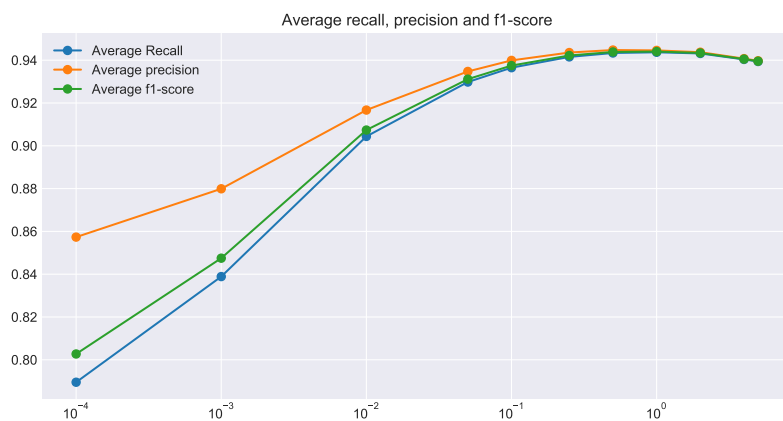
Figure 4.16: Optimal penalty parameters for linear svm when using SMOTE
