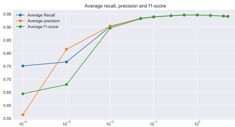
Figure 4.9: Optimal penalty parameters for linear svm
