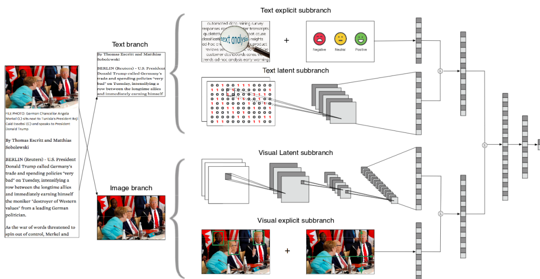
Figure 2.7: TI-CNN
