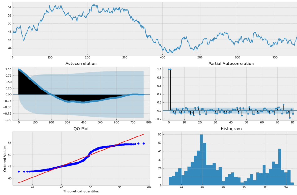
Figure 5.11 – Artificially generated random walk (AR(1) process). Noise sampled according to \epsilon \sim \mathcal{N}(-0.0178, 0.0991) with \xi_0 , \mu and \sigma^2 set to match the one of CAL2016.
