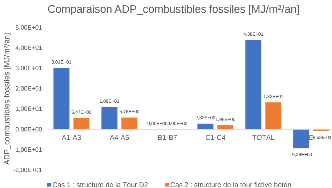
Figure 32 : Comparaison ADP_fossiles
