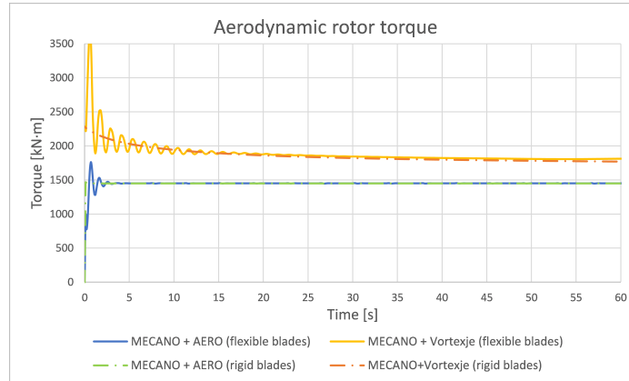
Figure 57: Dynamic response of the aerodynamic rotor torque.
